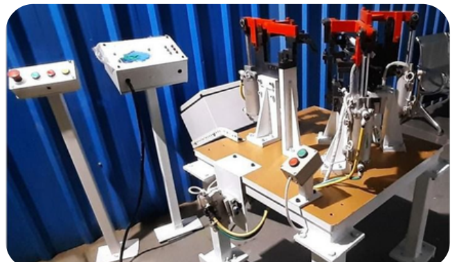
JIG & FIXTURE
