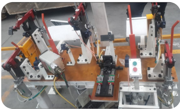
JIG & FIXTURE
