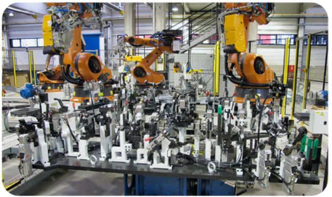
WELDING FIXTURE
